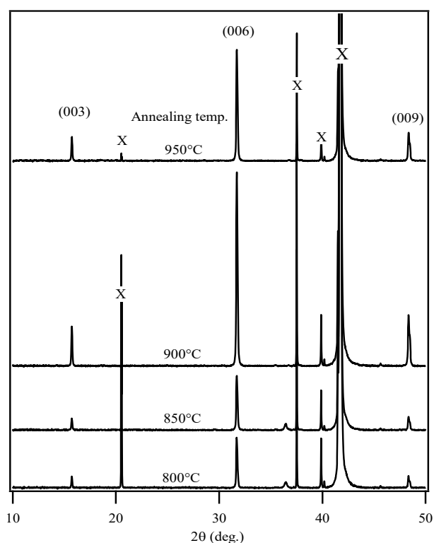
Fig. 2 XRD patterns of the films prepared on sapphire substrate using acetate precursor material. Peaks marked X are due to substrate.
