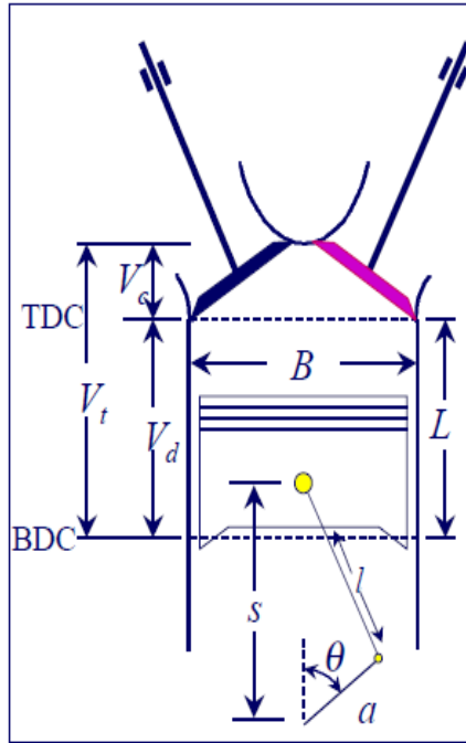
Fig. 3 An engine cylinder: l : The connecting rod length; a : the crank arm radius; B : the bore; s : the distance between crank axis and wrist pin axis; L : stroke length; V_c : The clearance volume; V_d : the displacement volume; V_t : the cylinder volume; TDC: top dead center; BDC: top bottom center
