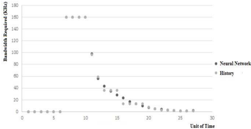
Fig. 7 Predicted exponential distribution for variable BW
