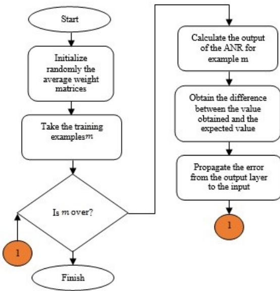
Fig. 2 MLPNN Training Diagram
