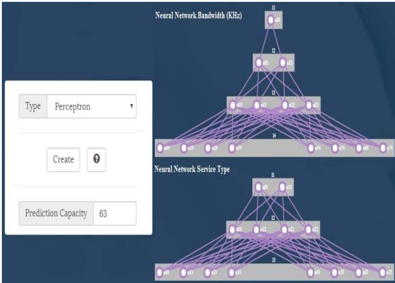
Fig. 4 Creation stage of the specialized MLPNNs
