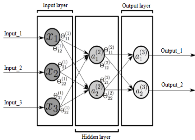
Fig. 1 Representation of the MLB for the data set of (5)
