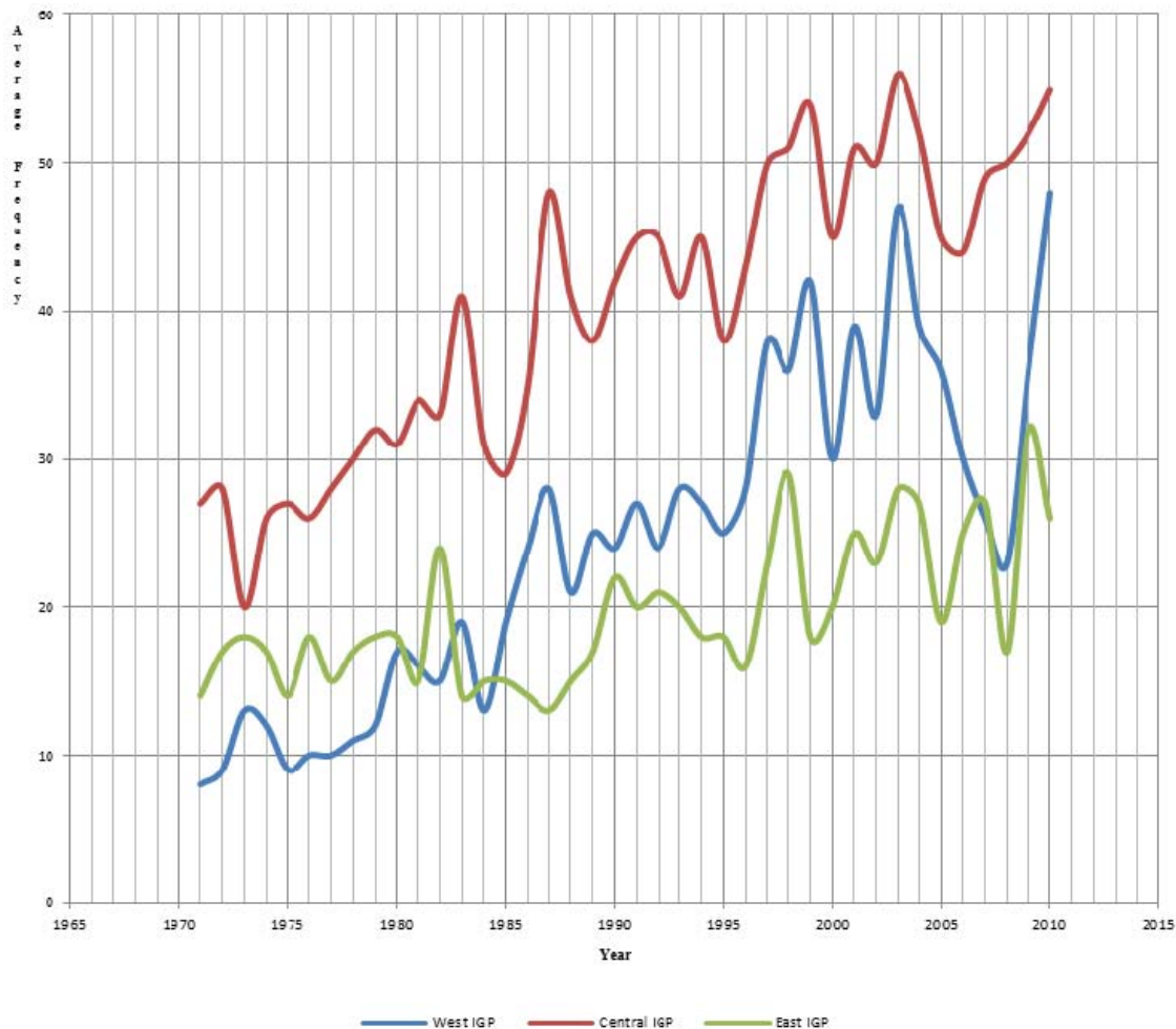
Fig. 7 Variation Points
