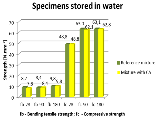
Fig. 2 Determination of strength of specimens stored in water
