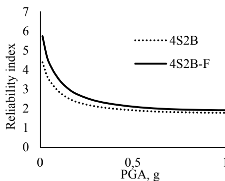
Fig. 7 Reliability curve – CP level
