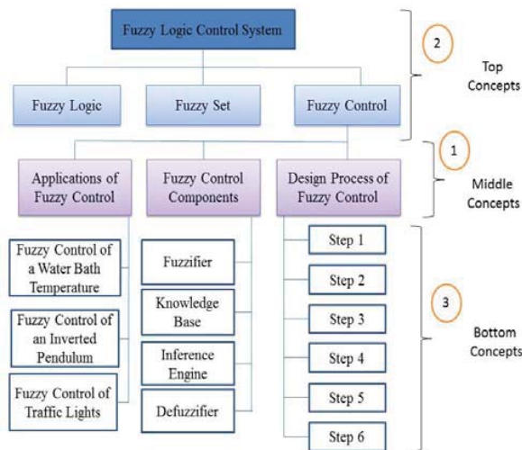
Fig. 4 Class hierarchy of FLC ontology
