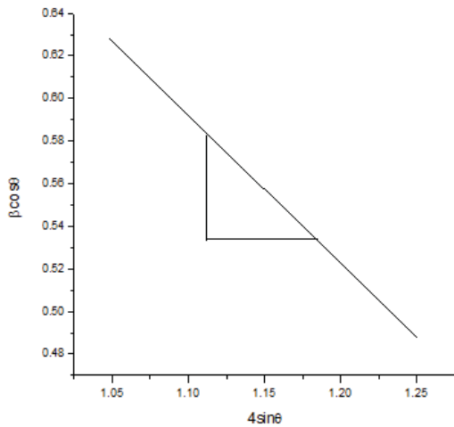
Fig. 2 Williamson-Hall plot
