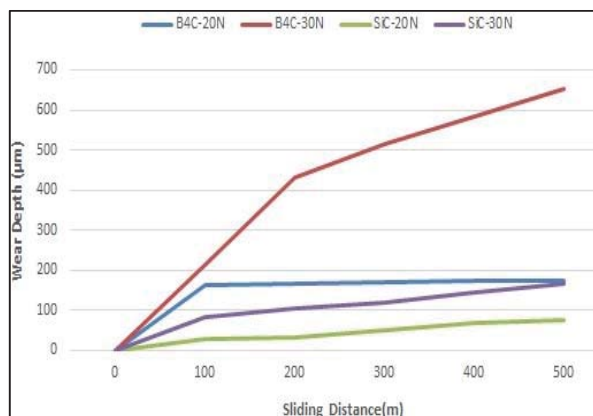
Fig. 3 Wear depth values of investigated composites
