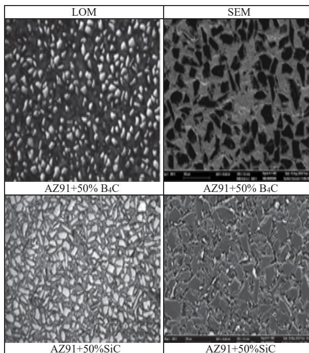
Fig. 2 Microstructure of investigated composites
