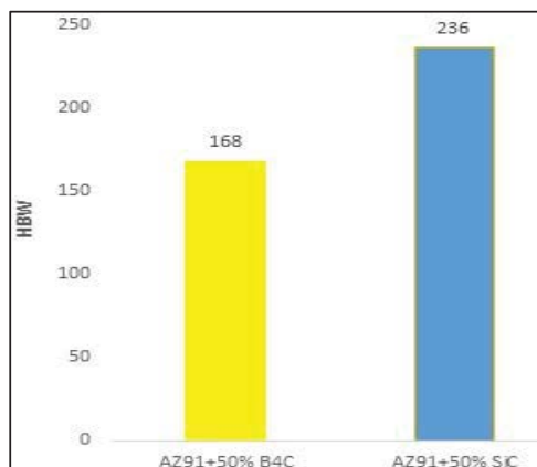
Fig. 1 Hardness values of investigated composites
