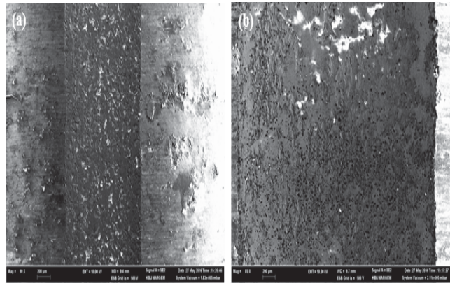
Fig. 6 SEM micrographs of the worn surfaces of (a) SiC90X (b) B 4 C 90X
