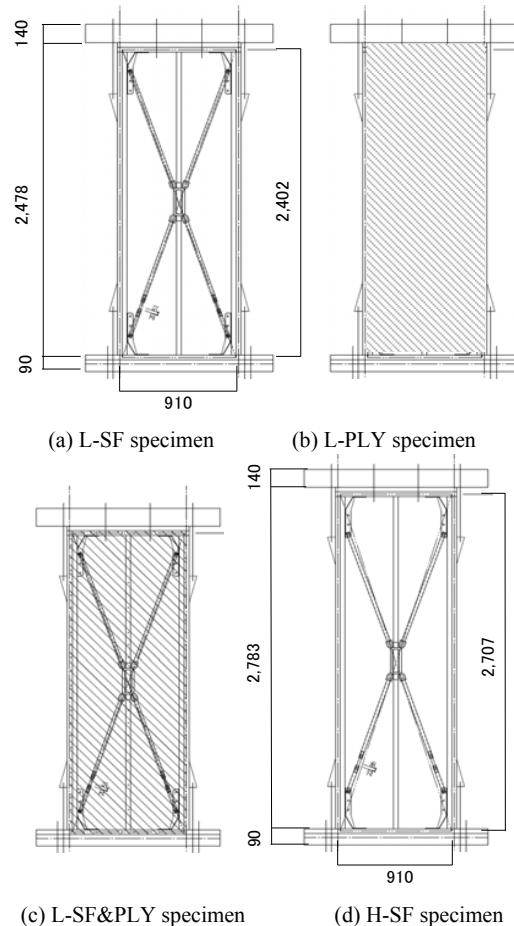
Fig. 6 Elevation of test frame specimens (unit: mm)
