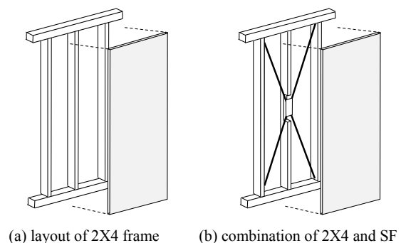
Fig. 5 Relation of two-by-four frame and SF structures
