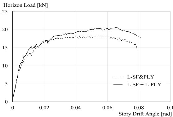
Fig. 10 Comparison of skeleton curve of L-SF&amp;PLY and summation of L-SF and L-PLY
