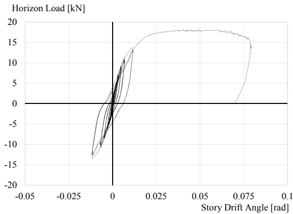
(c) L-SF&amp;PLY specimen
