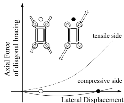
Fig. 4 Relation of axial force and lateral displacement
