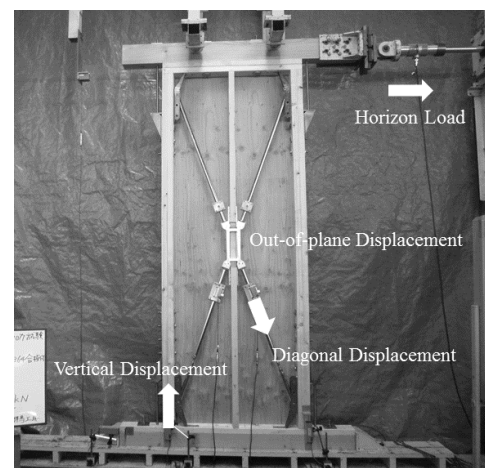
Fig. 7 Elevation of test setup and location of sensors
