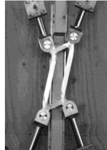
(a) plastic deformation of SF
