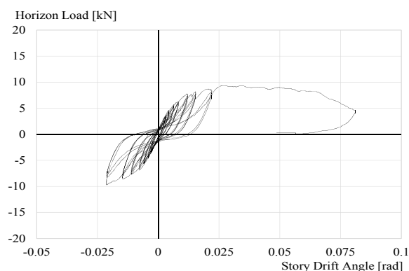
(b) L-PLY specimen
