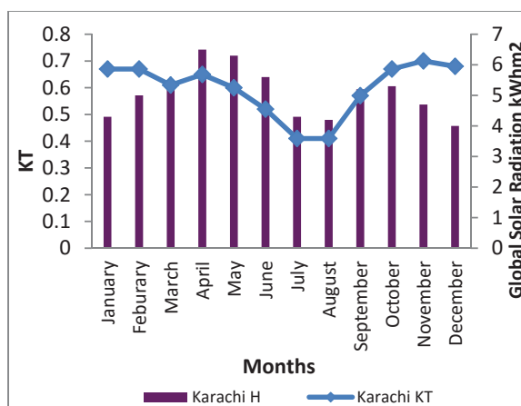
Fig. 6 Global Solar Radiation and Clearness Index for Karachi
