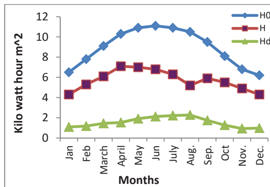
Fig. 4 Monthly variation of Extraterrestrial, Global and Diffuse solar radiation for Hyderabad, Sindh
