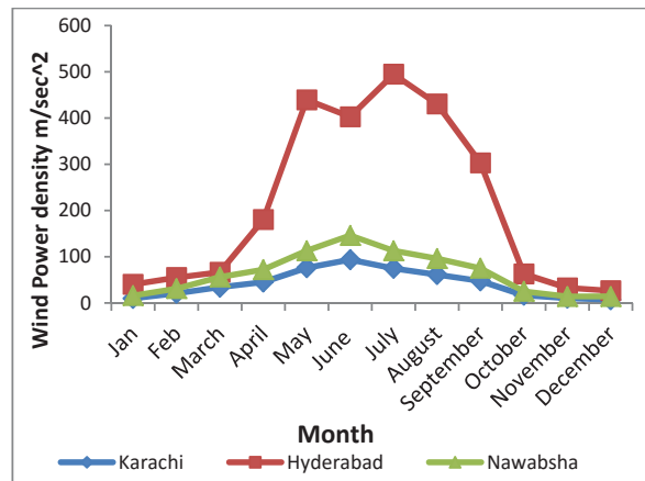
Fig. 10 Seasonal variation of wind power density at 10m height
