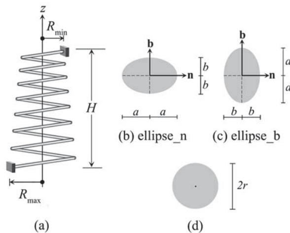
Fig. 1 Conical helix and cross-sectional geometries a = 5 \text{ mm} ,
