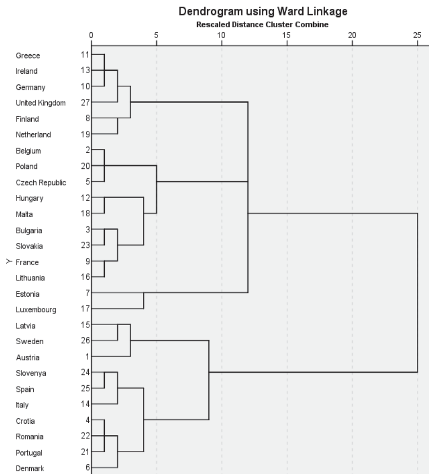
Fig. 4 Dendrogram using the Ward’s method
