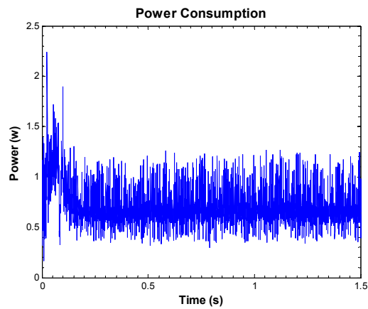
Fig. 18 Power consumption for hybrid method in the static mode
