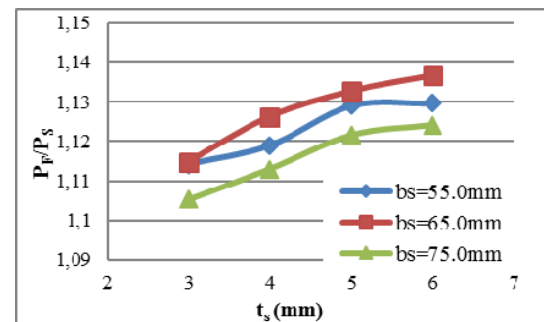
Fig. 9 Stiffener Thickness Vs Column Failure Load Ratio ( L/r = 100 , NS=4 & S/d_w = 0.93 )
