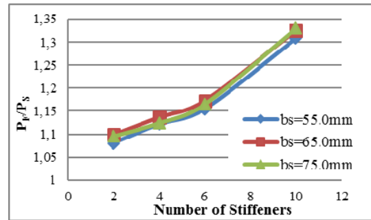
Fig. 23 Number of Stiffeners Vs Column Failure Load Ratio ( L/r=100 & t_s=6.0 mm)
