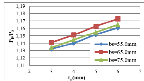
Fig. 10 Stiffener Thickness Vs Column Failure Load Ratio ( L/r = 100 , NS=6 & S/d_w = 0.67 )
