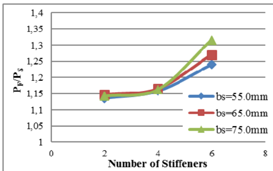
Fig. 17 Number of Stiffeners Vs Column Failure Load Ratio ( L/r=62.5 & t_s=4.0 mm)
