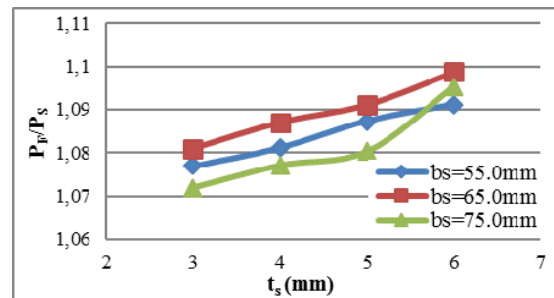
Fig. 8 Stiffener Thickness Vs Column Failure Load Ratio ( L/r = 100 , NS=2 & S/d_w = 1.56 )
