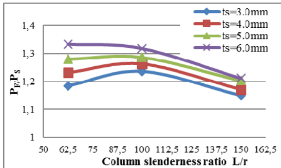
Fig. 39 Slenderness Ratio Vs Column Failure Load Ratio ( S/d_w=0.416 & b_s=55 mm)
