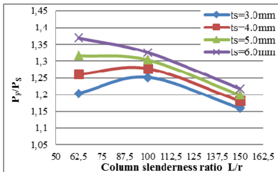
Fig. 40 Slenderness Ratio Vs Column Failure Load Ratio ( S/d_w=0.416 & b_s=65 mm)
