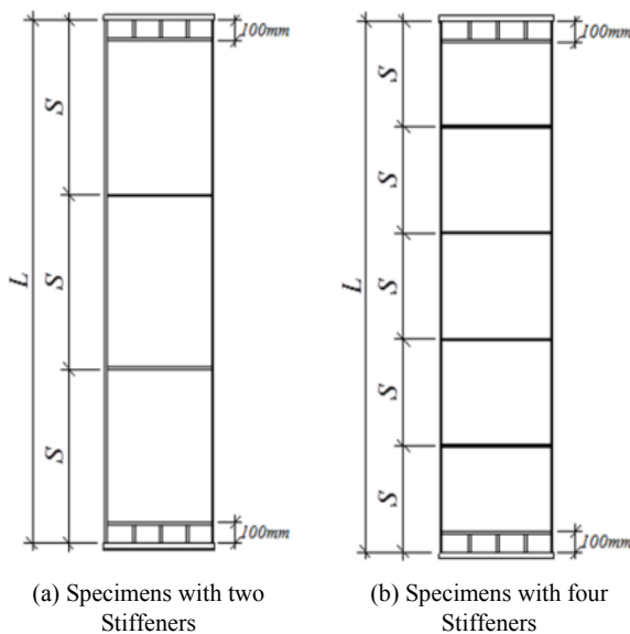
Fig. 1 Studied columns
