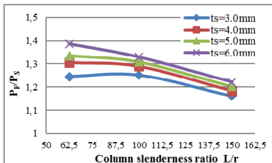
Fig. 41 Slenderness Ratio Vs Column Failure Load Ratio ( S/d_w=0.416 & b_s=75 mm)
