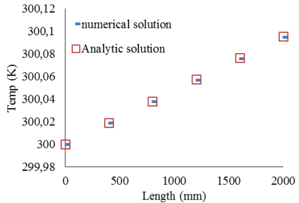
Fig. 4 Temperature profiles versus length of tube
