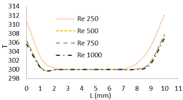
Fig. 9 Temperature and dimensionless velocity profiles at various Reynolds numbers at section (A)
