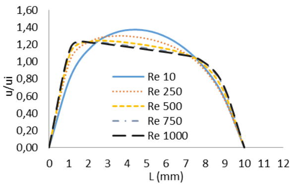
Fig. 8 Maximum velocity path at the curve section
