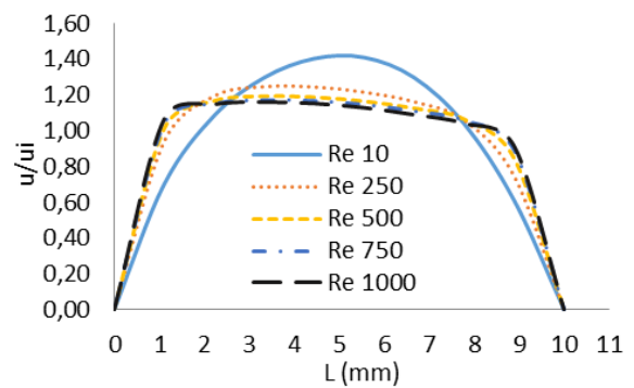
Fig. 8 Maximum velocity path at the curve section
