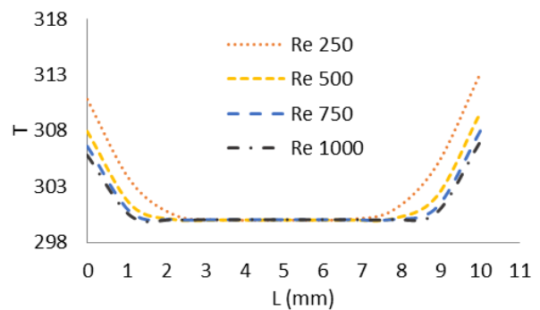
Fig. 10 Temperature and Dimensionless velocity profiles at various Reynolds numbers at section (B)
