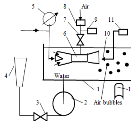
Fig. 1 Experimental setup
