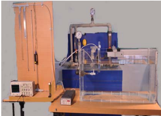
Fig. 2 Model of a laboratory rig
