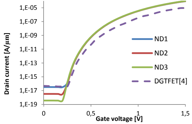
Fig. 3 Transfer characteristics of DGPNTFET and DGTfET [4] as a function of gate voltage. Here Si-pad donor doping ( N_D ) ( N_{D1}=1 \times 10^{15} \text{ cm}^{-3} , N_{D2}=1 \times 10^{16} \text{ cm}^{-3} , N_{D3}=1 \times 10^{17} \text{ cm}^{-3} )
