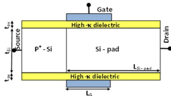
Fig. 1 Cross-sectional 2-D view of n-type Double gate PN diode based TFET (DGPNTFET) with high- \kappa gate dielectric: Width of the device is 1\mu m
