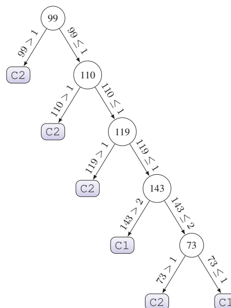
Fig. 3 Decision Tree from ENORA-DS
