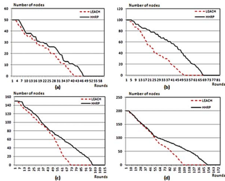
Fig. 4 Networks lifetime
