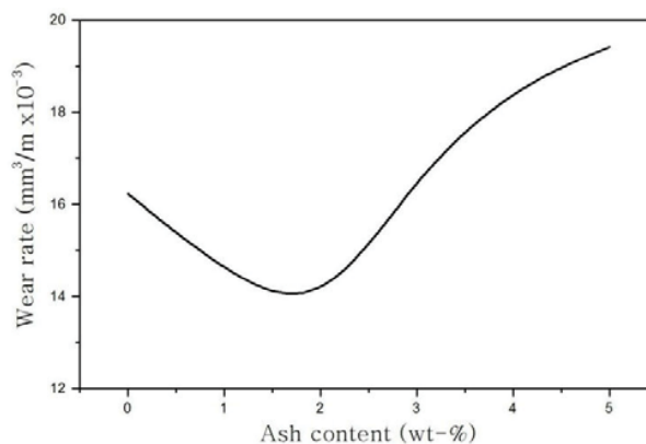
Fig. 5 Wear rate change as a function of ash content
