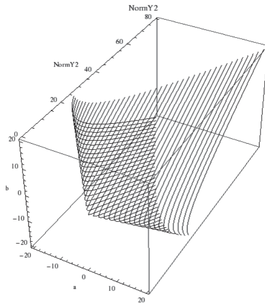
Fig. 15 Norms of Output Signal y_2 based on Corollary 1. R_2 form is a + bd . a and b range are -20 \leq a, b \leq 20
