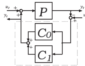
Fig. 5 Composite Stabilized Feedback with c_0 and c_1
