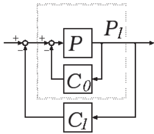
Fig. 4 Two-Stage Compensator Design ( y_2 to u_2 )
