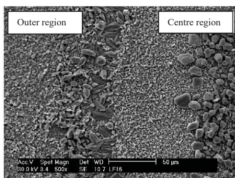
Fig. 2 SEM top surface between Sn-4Ag-0.5Cu-xBi and Ni/Au surface finish showing “beach mark”
