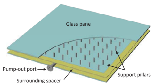
Fig. 8 Schematic diagram of a flat vacuum panel
