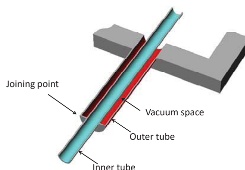
Fig. 3 Schematic diagram of co-centric tube inlet and outlet port design
