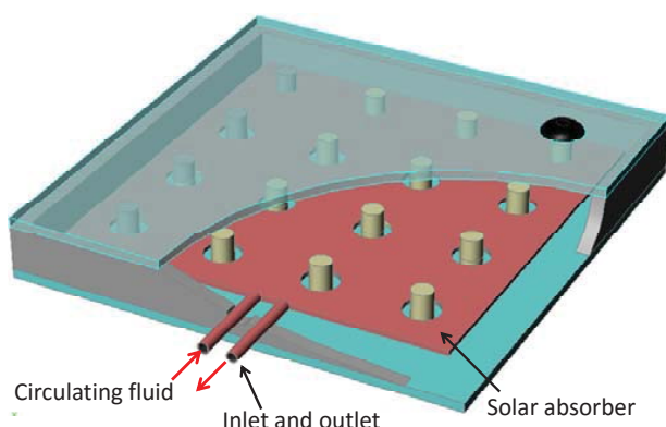
Fig. 2 Schematic diagram of a flat vacuum panel
