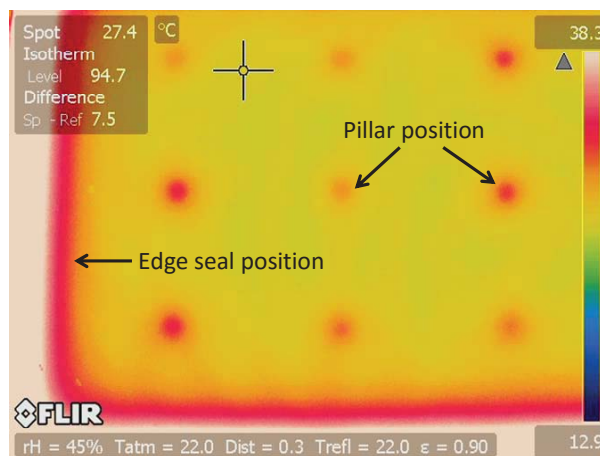
Fig. 7 IR-image of a flat vacuum panel
