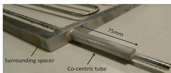
Fig. 4 Co-centric tube inlet and outlet port design
