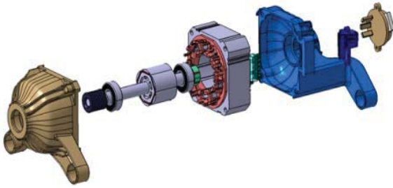
Fig. 2 Structure of BLDC Motor for Washing machine
