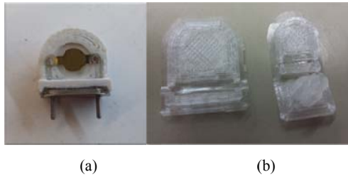
Fig. 3 Image of the version V2.0 holder (a) ABS polymer holder (b) Bentlay® holder
