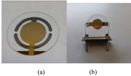
Fig. 4 Image of the ICM sensors used (a) INFICON 1" (b) ICM ½"
