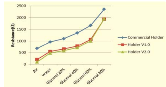
Fig. 6 Resistance measurements (in Ω) for different liquids media and holders, using the ICM Crystal
