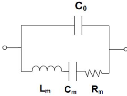
Fig. 1 Butterworth-van Dyke model of Quartz Crystal Resonator
