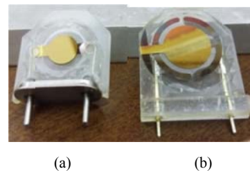
Fig. 2 Image of the version V1.0 methacrylate holder (a) ICM \frac{1}{2} " sensor (b) INFICON 1" sensor
