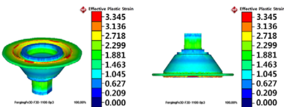
Fig. 5 Simulation results of effective plastic strain after hot forging at 1,100°C
