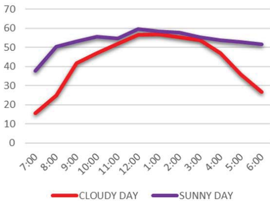
Fig. 4 Power output values obtained by the tracker
