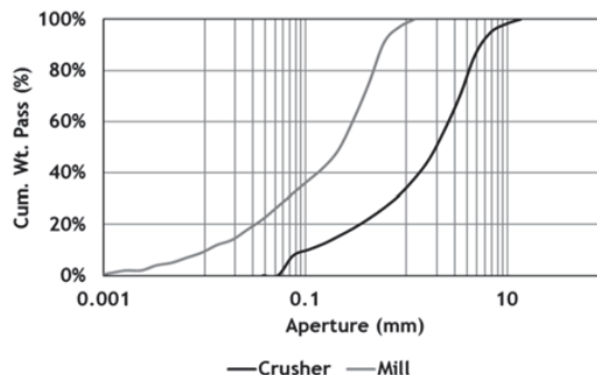
Fig. 2 Comparison between crushed ore and milled ore
