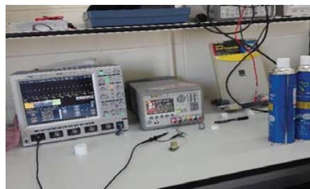
Fig. 2 Performance Test of gas sensor modules
