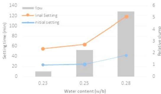
Fig. 3 Effect of water content on Flowability and setting time of geopolymer mortar
