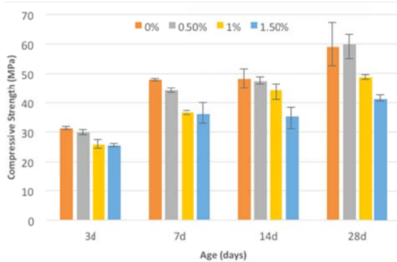
Fig. 6 Effect of superplasticizer content on the compressive strength of geopolymer mortar
