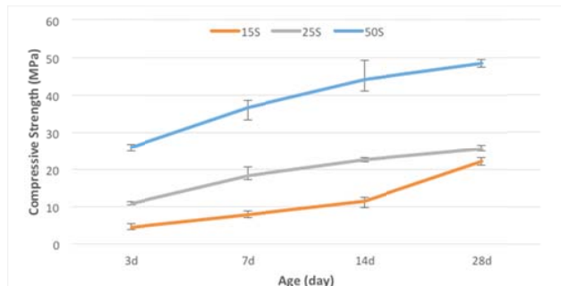
Fig. 7 Effect of alkaline activator on the compressive strength of geopolymer mortar
