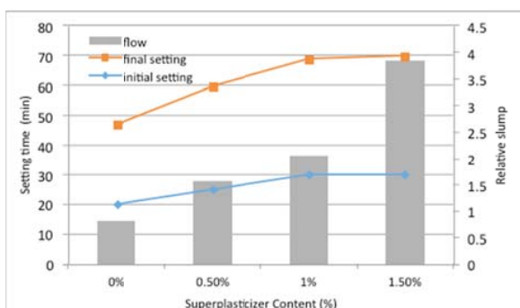
Fig. 4 Effect of superplasticizer contents on the flowability and setting time of geopolymer mortar
