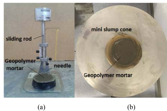
Fig. 2 (a) Setting time apparatus, (b) Flowability measurement
