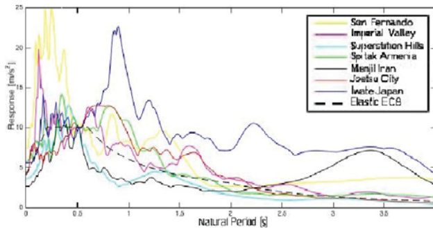
Fig. 7 Response spectrum of selected ground motions
