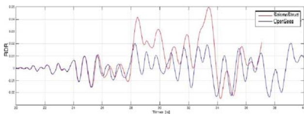
Fig. 10 Displacement response of the control node for "Iwate Japan"-ground motion increased by 50 %
