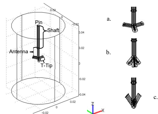
Fig. 1 The configurations of the geometry model of the T-Prong monopole antennas: (a) Three T-prong Monopole (3TP), (b) Expand T-Prong antenna (ETP) and (c) Arrow T-Prong antenna (ATP)
