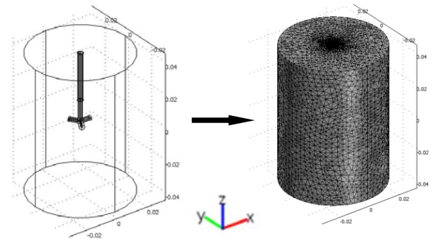
Fig. 2 The cross-section of the meshed model
