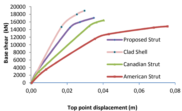
(b) Static nonlinear analysis Y-Y
