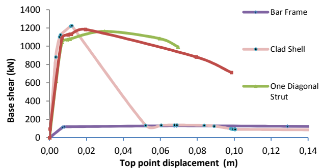
Fig. 10 Pushover curves for no infill model (bare frame only), Layered shell infill model, and proposed strut infill model (one diagonal or cross diagonal), t=0.25m
