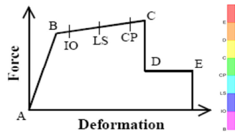
Fig. 7 Generalized force-deformation relation for elements or components
