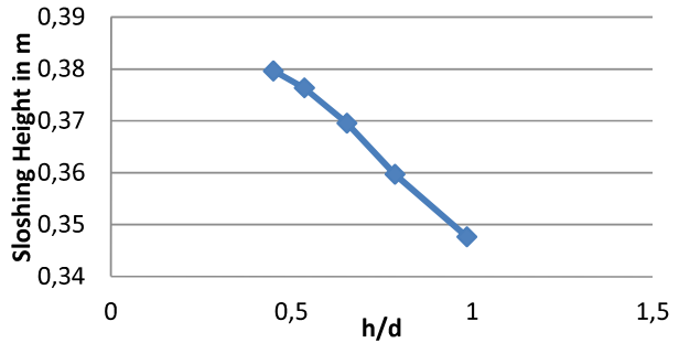
Fig. 20 Variation of Maximum Sloshing Height with h/d (200 KL)
