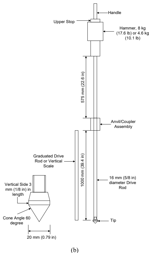
Fig. 1 (a) Soil Stiffness Gauge and (b) Dynamic Cone Penetrometer
