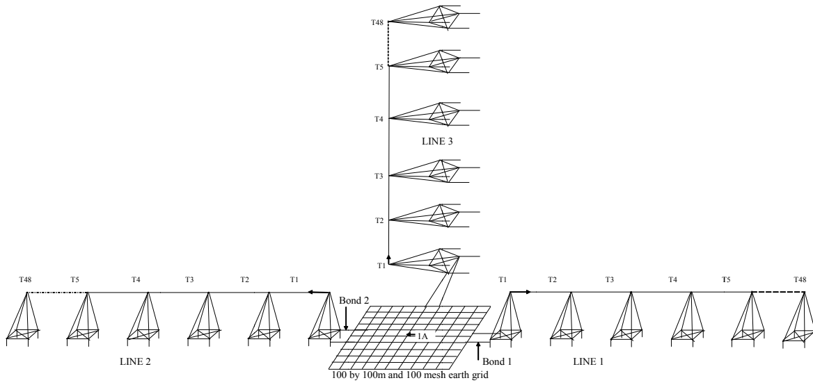
(a) Schematic model used in simulations
