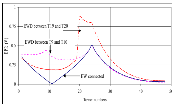
Fig. 9 Effect of break in earth wire on EPR at tower bases (Model 3)
