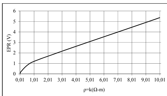
Fig. 3 Computed earth potential rise for a healthy system (Model 1, Scenario I)
