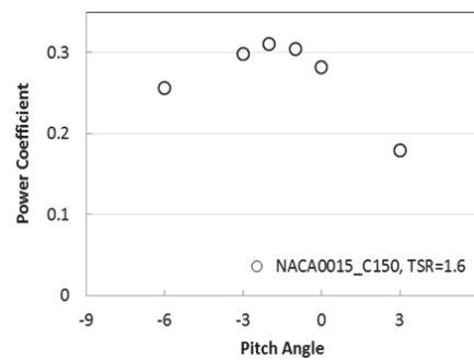
Fig. 8 Variations of power coefficients at varying pitch angles
