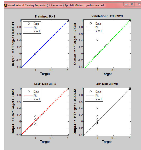
Fig. 7 Training Regression Plot
