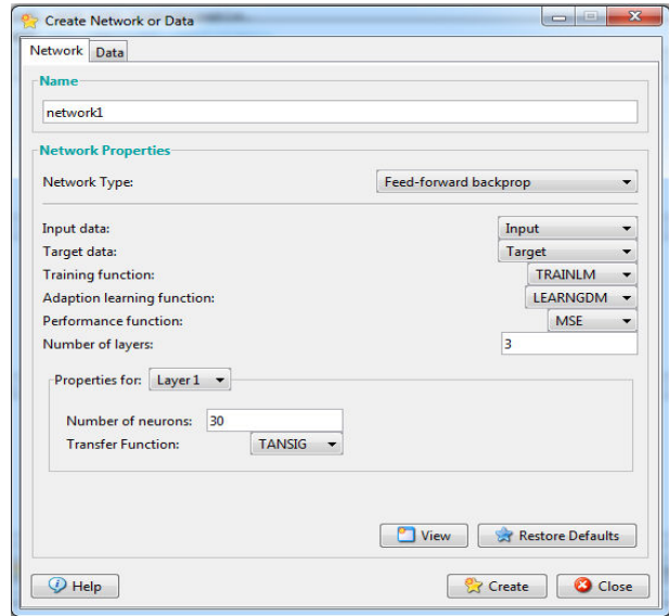
Fig. 2 Creation of Neural Network
