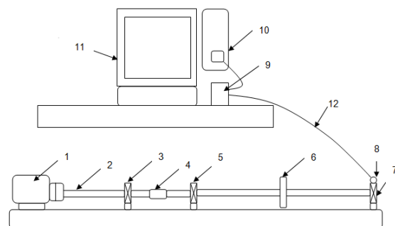
Fig. 1 Experimental Setup [10]
