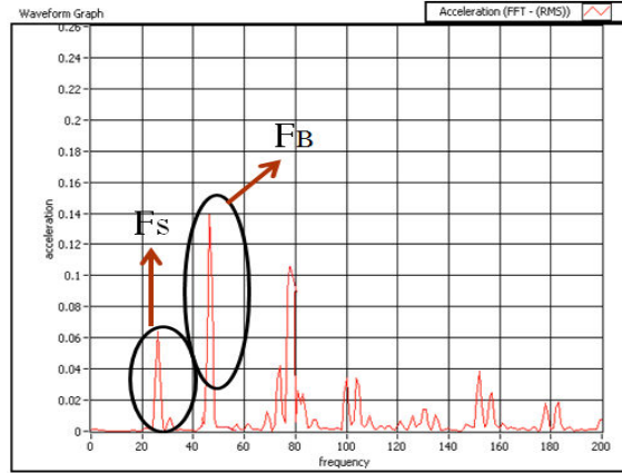
Fig. 5 Spectrum of Ball defect bearing
