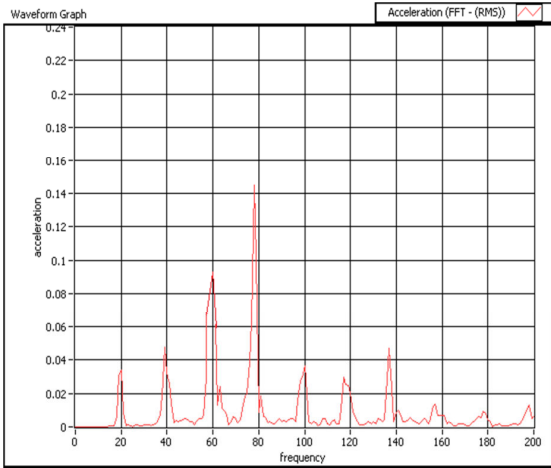
Fig. 3 Spectrum of Good bearing
