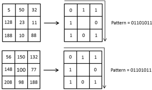
Fig. 1 An example of drawback of LBP
