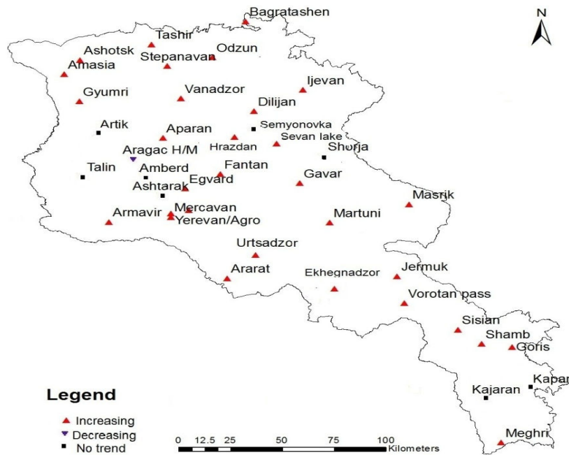
Fig. 1 Rank correlation tests results (point data)
