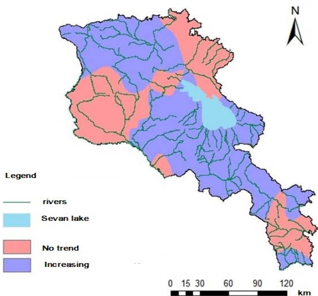
Fig. 6 Mann-Kendall test for average annual temperature over the period 1961-2012 (interpolated results)
