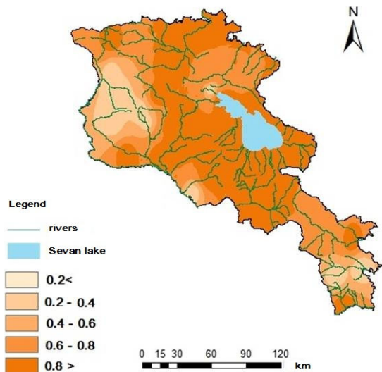
Fig. 3 Hubert segmentation tests results
