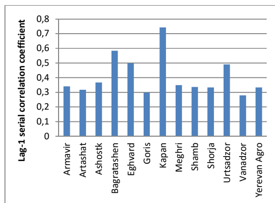
Fig. 4 Lag-1 serial correlation coefficient for the meteorological variables at the weather stations for temperature
