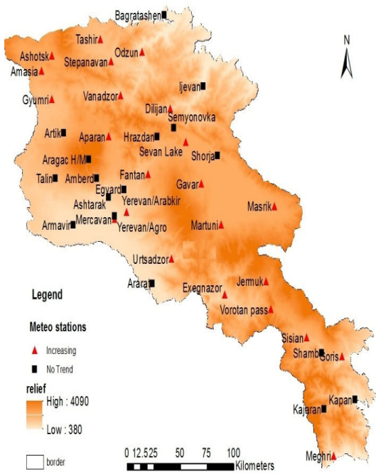
Fig. 5 Mann-Kendall test for average annual temperature over the period 1961-2012 (point data)
