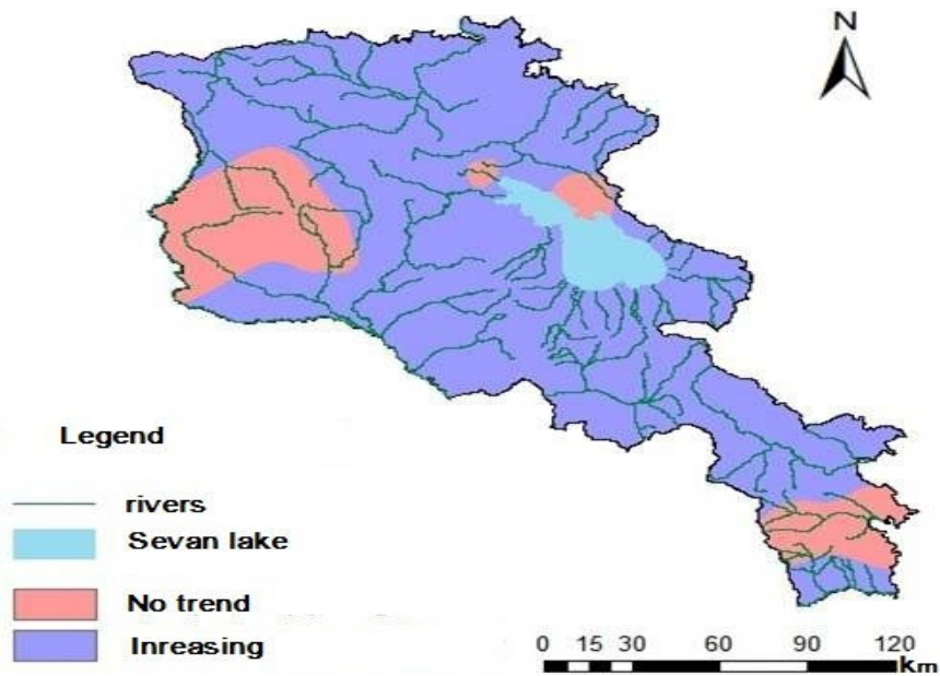
Fig. 2 Rank correlation tests results (interpolated results)
