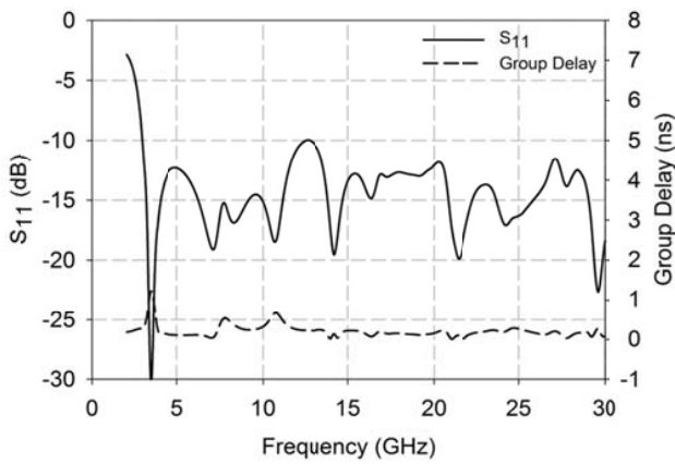
Fig. 3 Simulated return loss and group delay response against frequency of the proposed broadband antenna.
