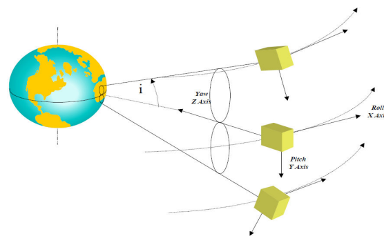
Fig. 6 Satellite pointing in inclined orbit configuration
