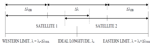
Fig. 2 EW Dead band for longitude Separation Strategy; 2\Delta\lambda_{TOL} = \Delta\lambda + 2\Delta\lambda_{DB} , \Delta\lambda is the separation between satellites
