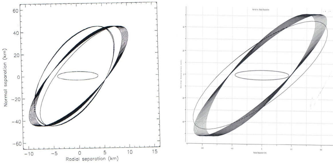
Fig. 10 Two Cases of circle violation corrections for Satellite X, Y
