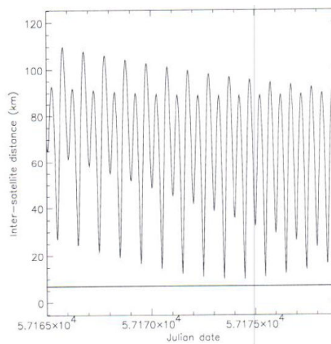
Fig. 17 Adjustment of the "normal_vs_radial separation" circle and min inter-satellite distance
