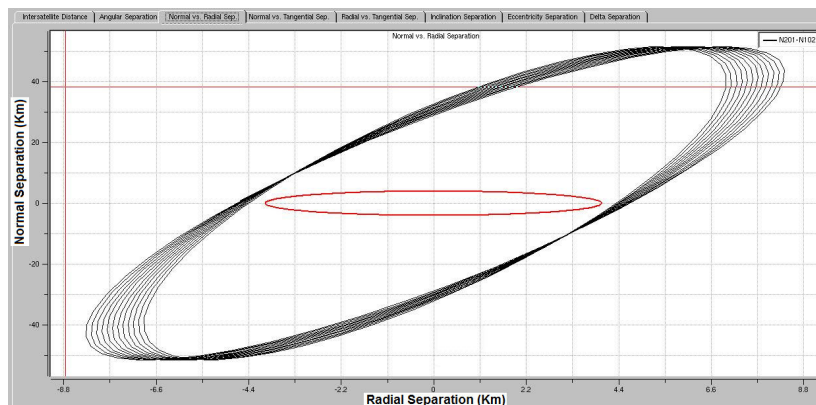
Fig. 12 "Normal_vs_radial separation" circle with NO maneuver
