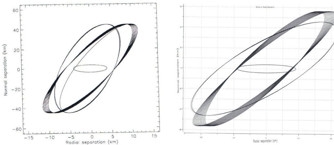
Fig. 9 Two Cases of circle violation for Satellite X, Y
