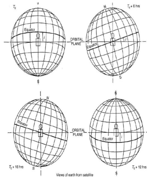
Fig. 5 Satellite inclination-induced Yaw Variation along the orbit
