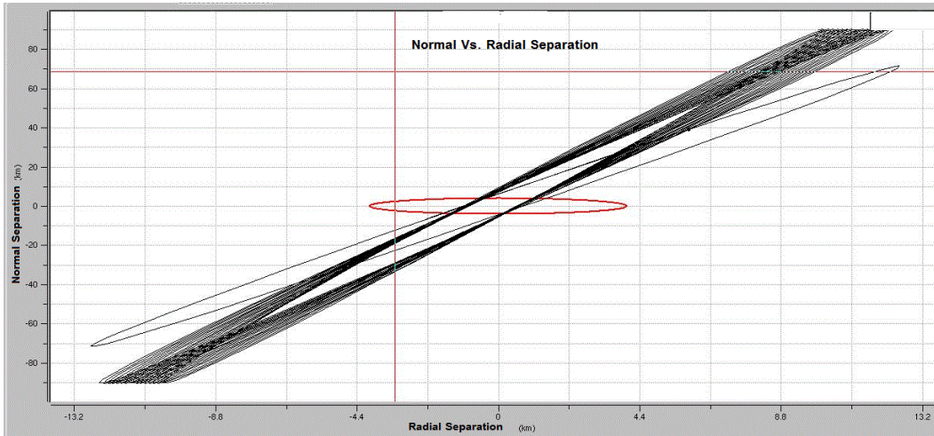
Fig. 7 Violation of the "Normal_vs_Radial separation" circle
