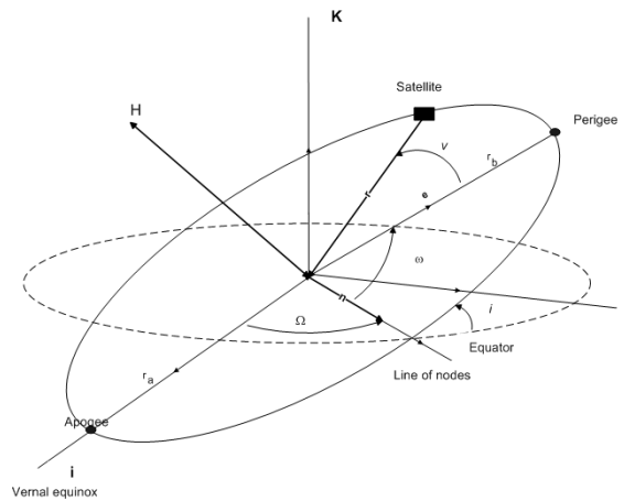
Fig. 1 Orbital angles
