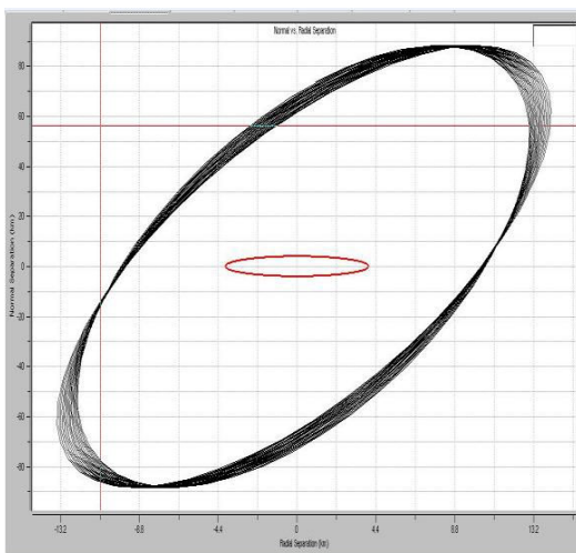
Fig. 17 Adjustment of the "normal_vs_radial separation" circle and min inter-satellite distance
