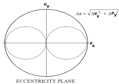
Fig. 3 EW Dead band for Eccentricity Separation Strategy
