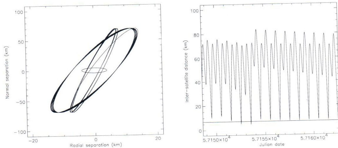
Fig. 15 (c) Scenario 3 – Change e_x and e_y and ecc radius
