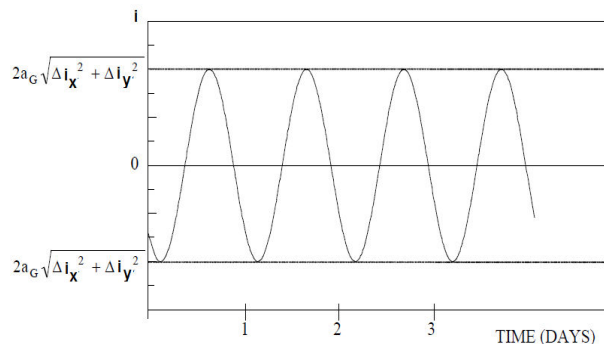
Fig. 4 Motion along the 'i' axis with Inclination Separation Strategy
