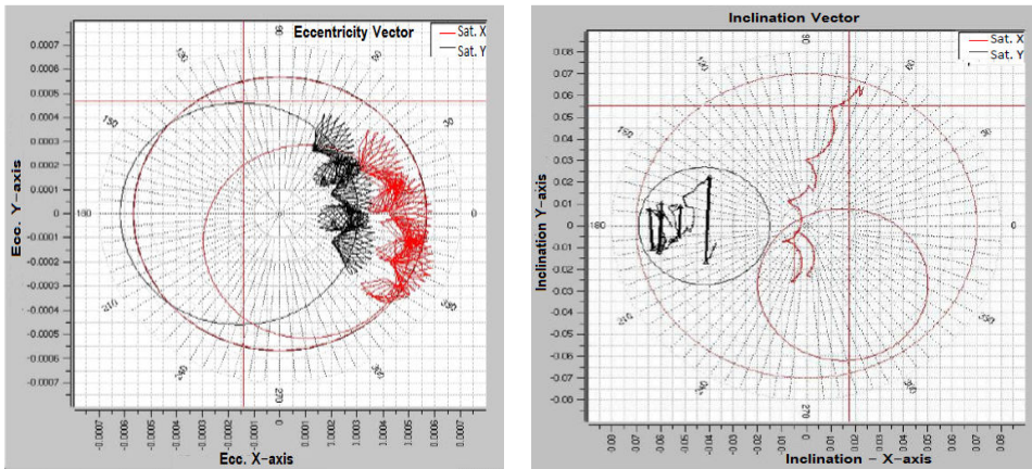
Fig. 7 Violation of the "Normal_vs_Radial separation" circle
