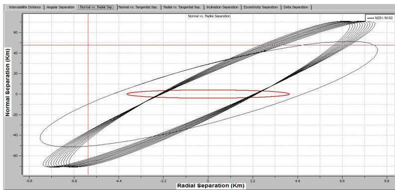
Fig. 11 Case of circle violation for Satellite X, Y
