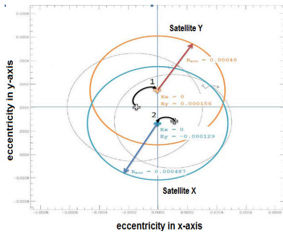
Fig. 16 New control circle adjustment
