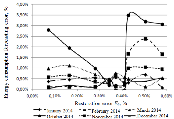
Fig. 2 Dependency diagrams of the energy consumption forecasting error \sigma_{pr} and the restoration error E_0
