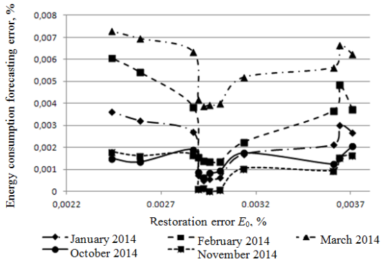
Fig. 1 Dependency diagrams of the energy consumption forecasting error \sigma_{pr} and the restoration error E_0
