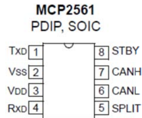
Fig. 1 CAN Transceiver
