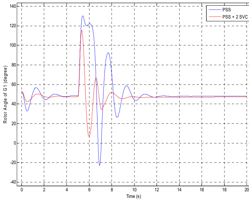
Fig. 18 Rotor angle difference of G1 to G2
