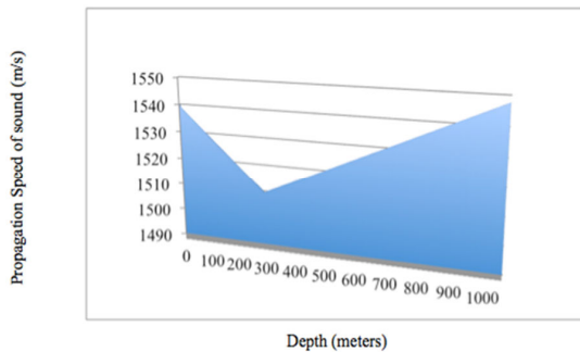
Fig. 1 Propagation speed vs. Depth
