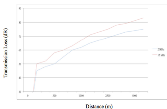
Fig. 4 Transmission loss vs distance
