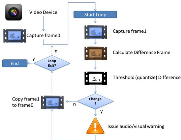
Fig. 1 Change detection Algorithm
