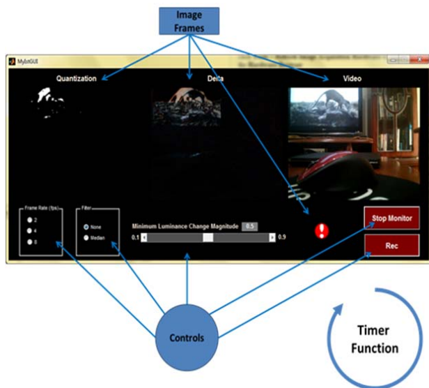
Fig. 4 System's GUI
