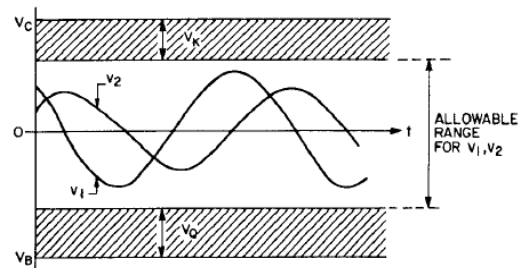
Fig. 2 Terminal voltages for the transistor [1]
