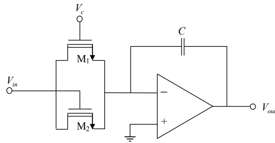
Fig. 11 MOS-C realization of Miller integrator [7]
