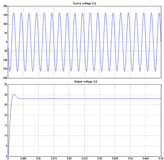
Fig. 20 Charts operation AC-DC converter
