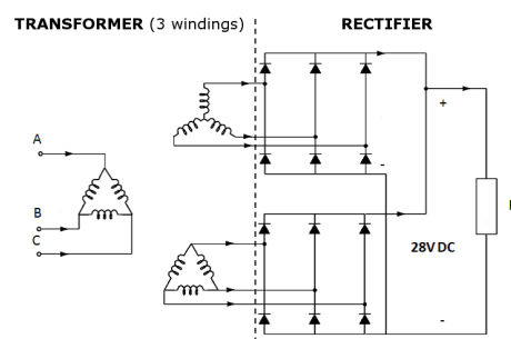
Fig. 7 Diagram of AC-DC rectifier on civil aircraft
